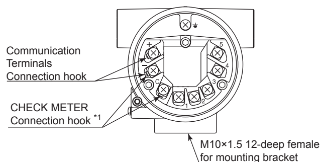
Terminal Configuration
